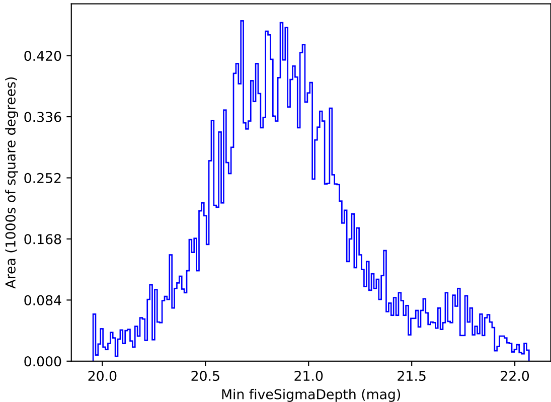
too_elab_r8_d2_giz_v3.4_10yrs All sky all bands: Min fiveSigmaDepth
