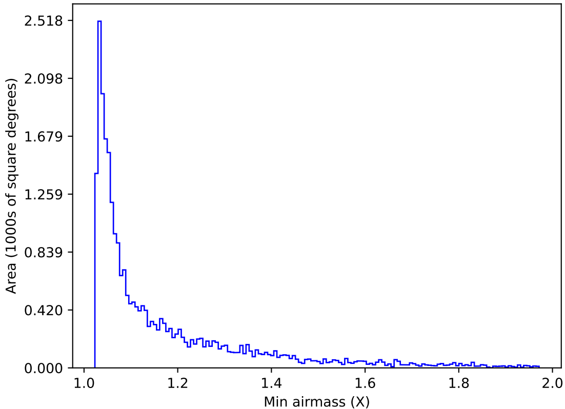
too_elab_r8_d2_giz_v3.4_10yrs Yr 1 z band: Min airmass
