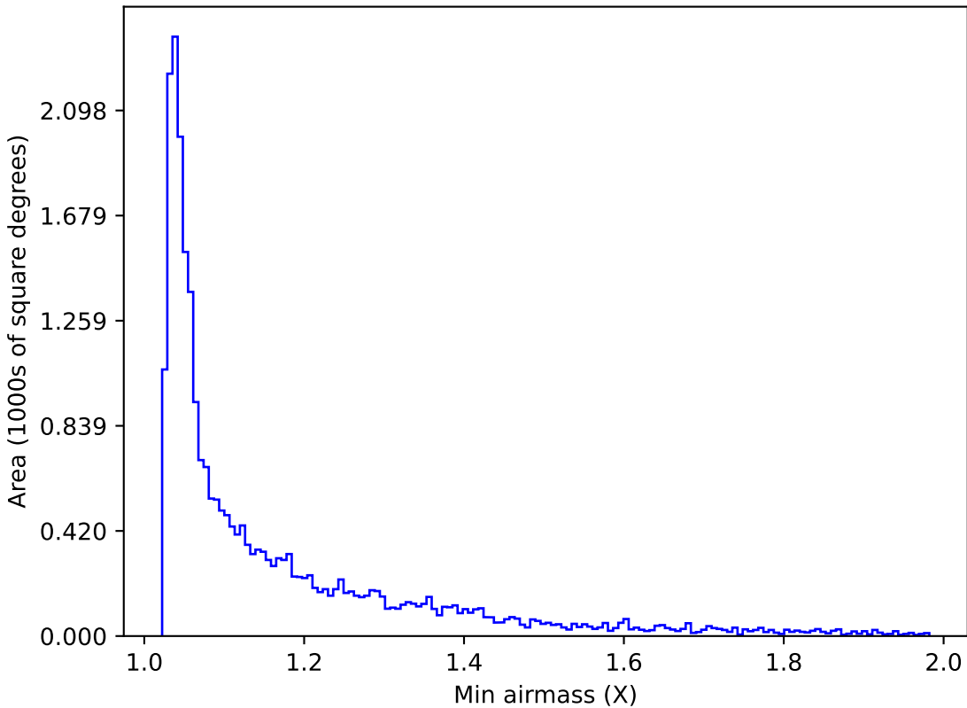
too_elab_r8_d2_giz_v3.4_10yrs Yr 1 z band: Min airmass
