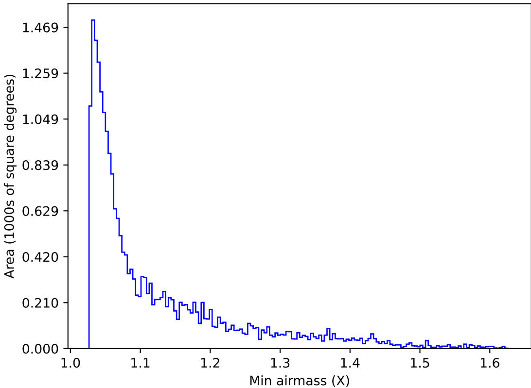
too_elab_r8_d2_giz_v3.4_10yrs Yr 1 y band: Min airmass
