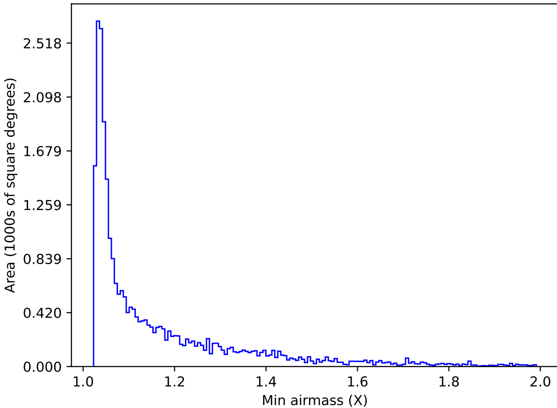
too_elab_r8_d2_giz_v3.4_10yrs Yr 1 r band: Min airmass
