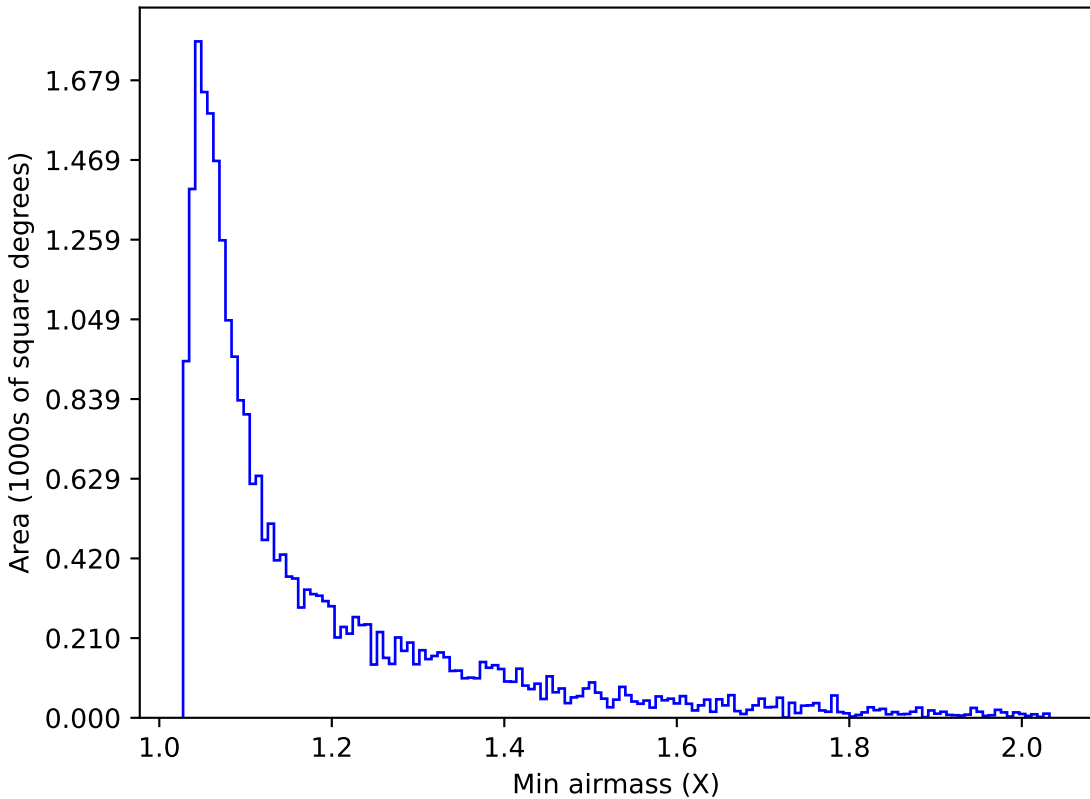
too_elab_r8_d2_giz_v3.4_10yrs Yr 1 g band: Min airmass
