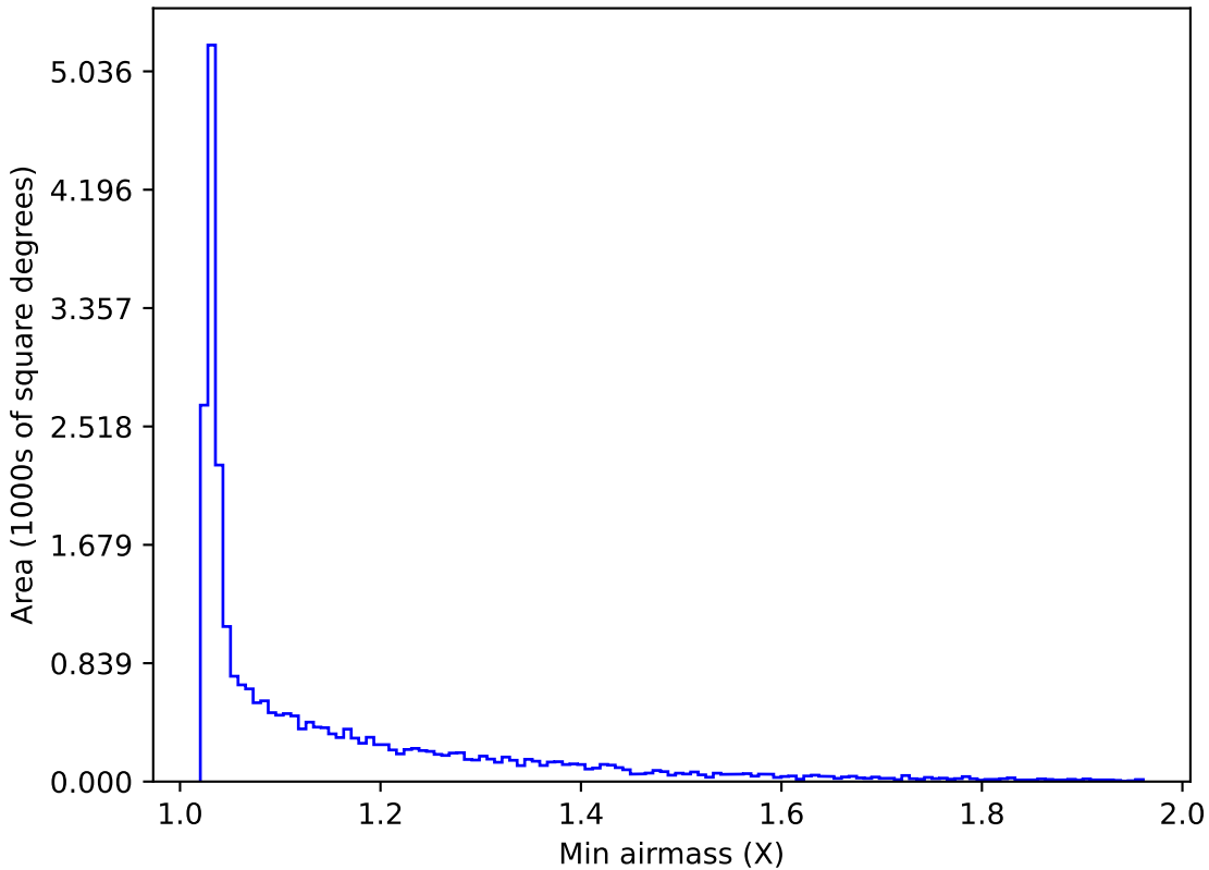
too_elab_r8_d2_giz_v3.4_10yrs Yr 1 all bands: Min airmass
