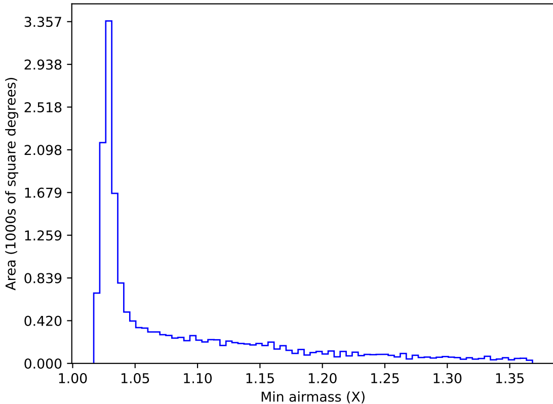
too_elab_r8_d2_giz_v3.4_10yrs WFD z band: Min airmass
