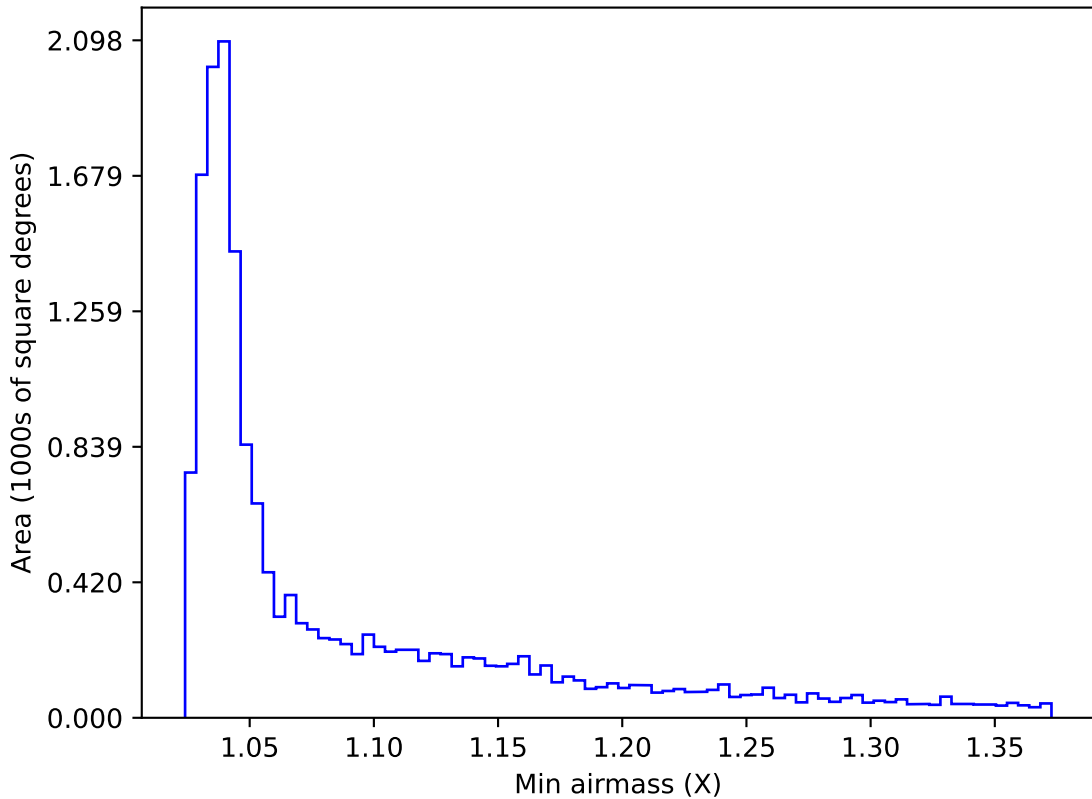
too_elab_r8_d2_giz_v3.4_10yrs WFD u band: Min airmass
