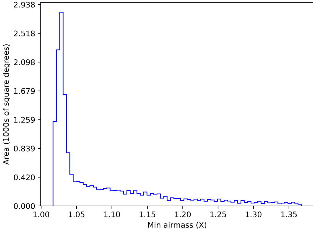
too_elab_r8_d2_giz_v3.4_10yrs WFD r band: Min airmass
