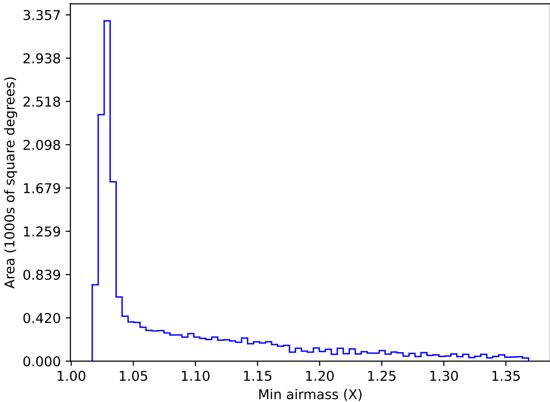
too_elab_r8_d2_giz_v3.4_10yrs WFD i band: Min airmass
