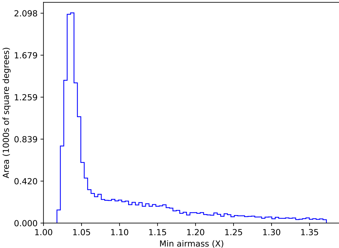
too_elab_r8_d2_giz_v3.4_10yrs WFD g band: Min airmass
