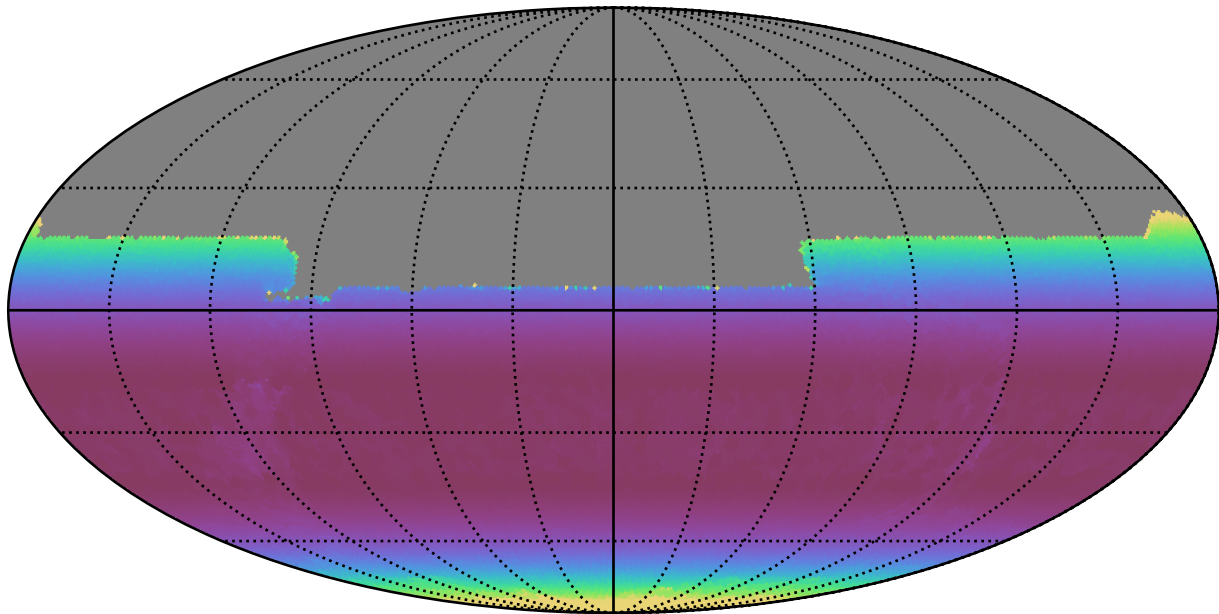
too_elab_r8_d2_giz_v3.4_10yrs All sky y band: Min airmass
