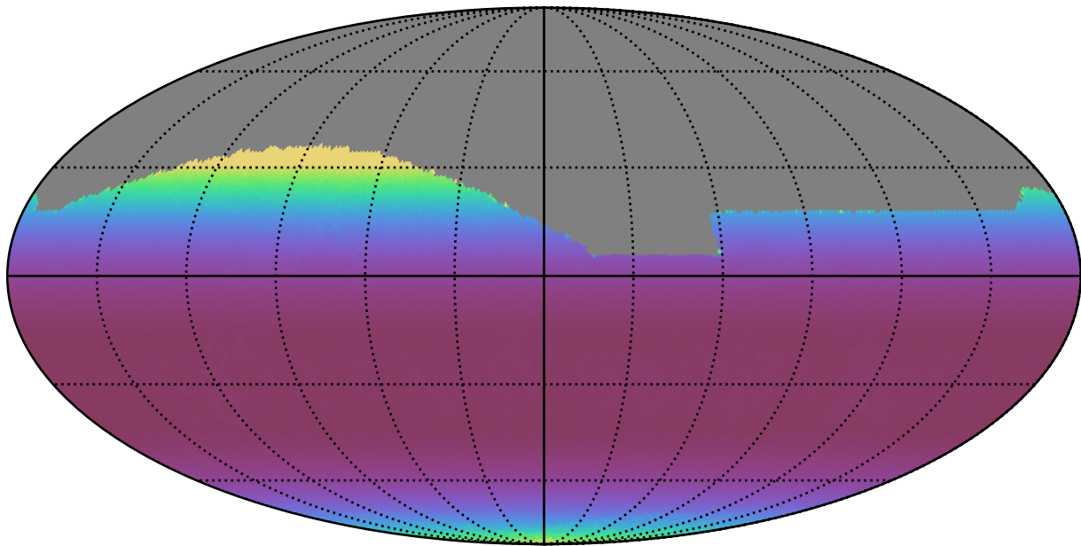
too_elab_r8_d2_giz_v3.4_10yrs All sky r band: Min airmass
