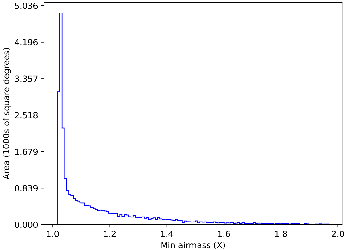
too_elab_r8_d2_giz_v3.4_10yrs All sky r band: Min airmass
