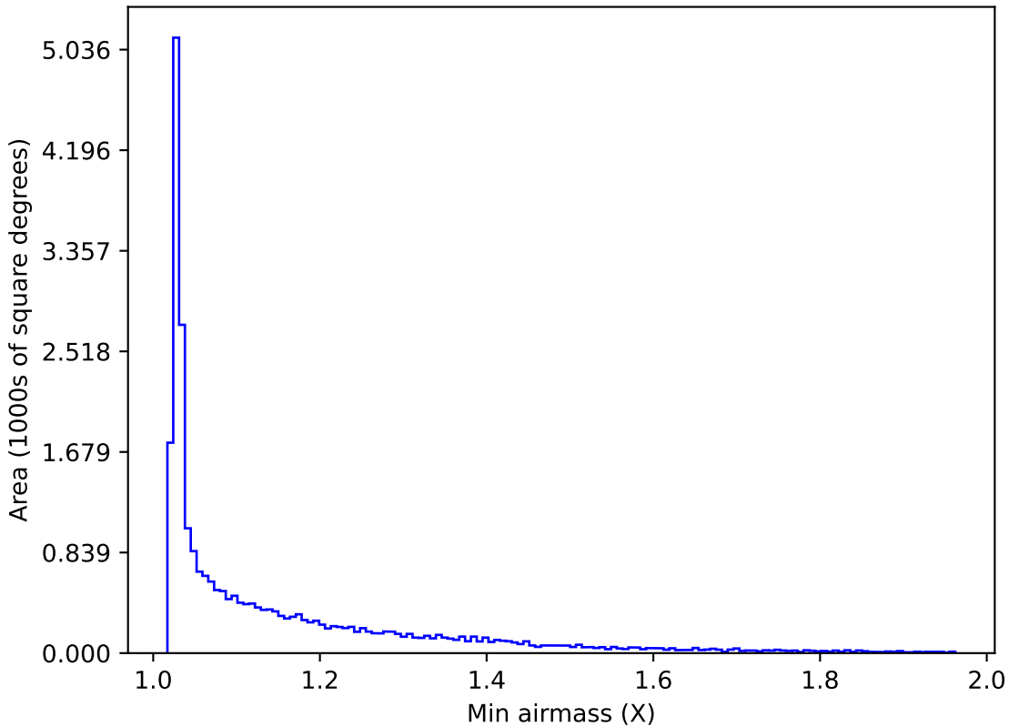
too_elab_r8_d2_giz_v3.4_10yrs All sky i band: Min airmass
