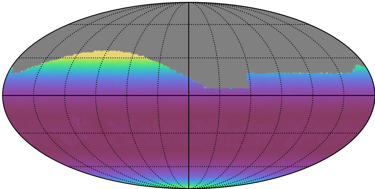
too_elab_r8_d2_giz_v3.4_10yrs All sky g band: Min airmass
