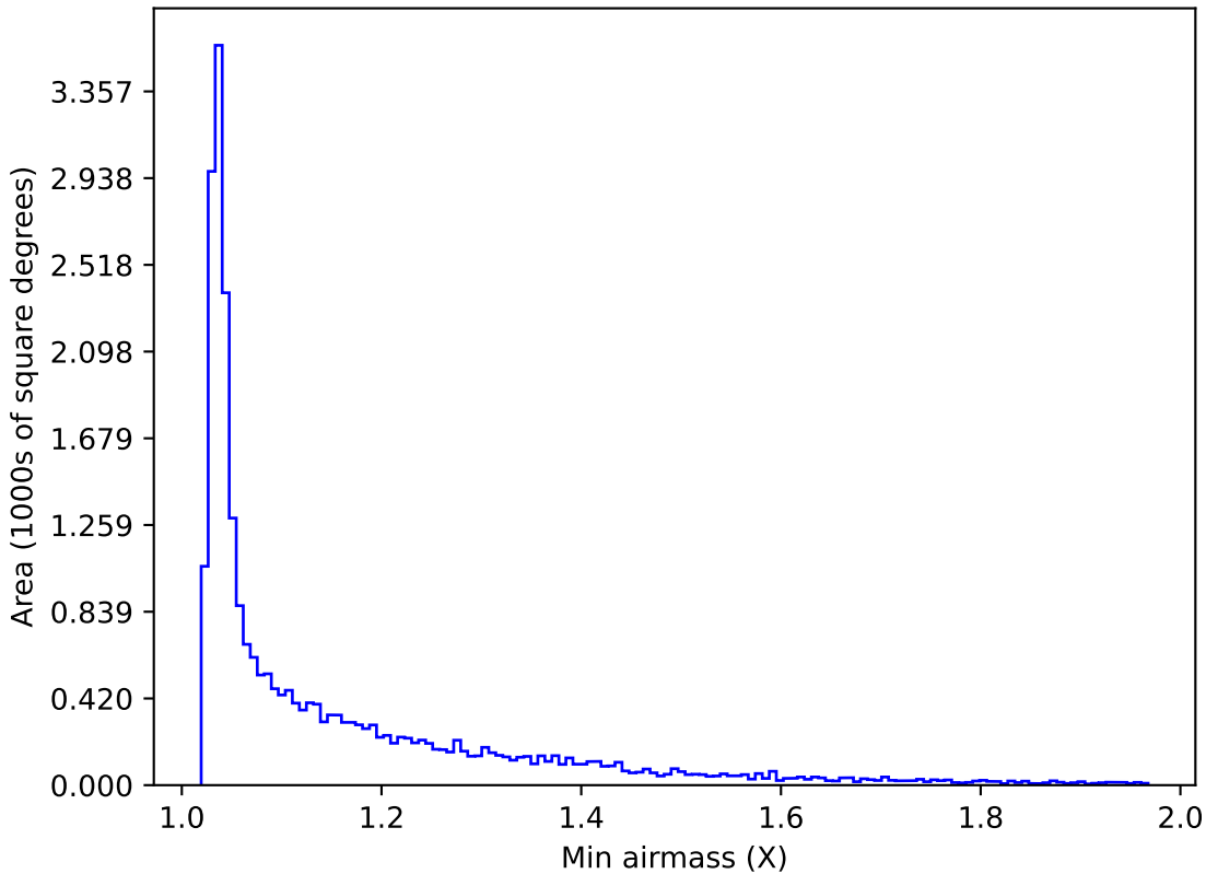
too_elab_r8_d2_giz_v3.4_10yrs All sky g band: Min airmass
