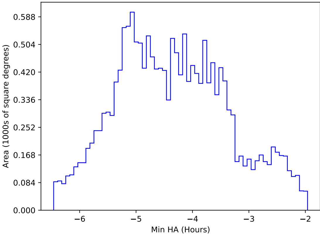
too_elab_r8_d2_giz_v3.4_10yrs WFD z band: Min HA
