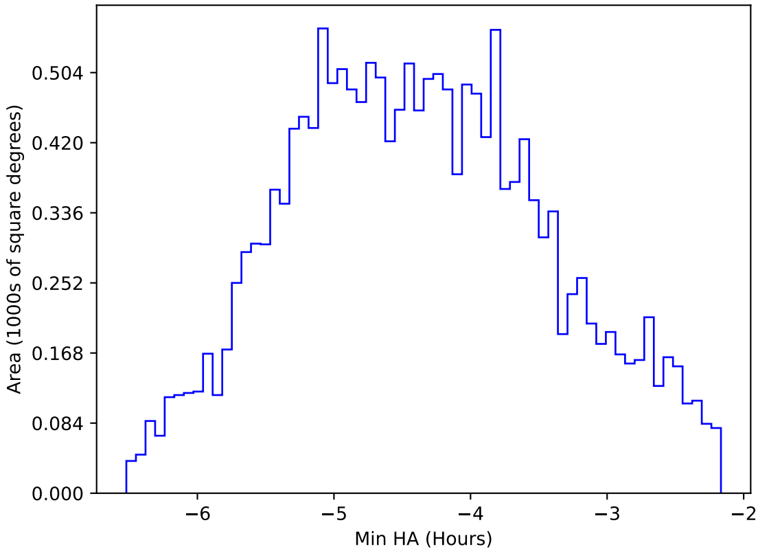
too_elab_r8_d2_giz_v3.4_10yrs WFD z band: Min HA
