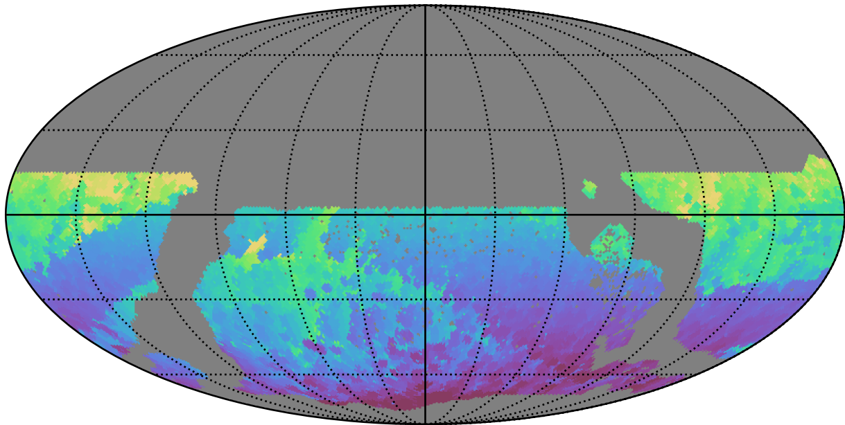
too_elab_r8_d2_giz_v3.4_10yrs WFD r band: Min HA
