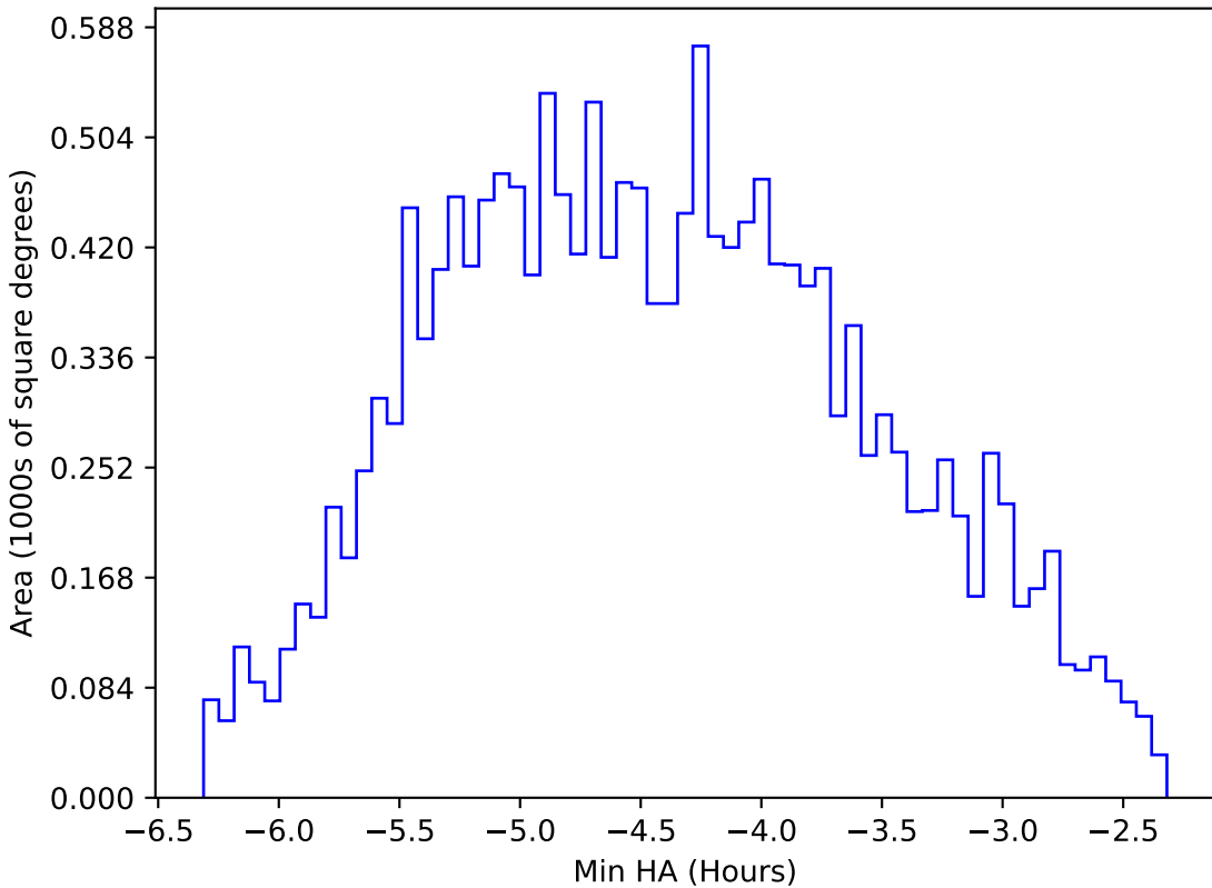
too_elab_r8_d2_giz_v3.4_10yrs WFD r band: Min HA
