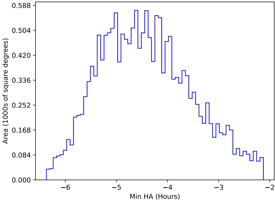
too_elab_r8_d2_giz_v3.4_10yrs WFD r band: Min HA
