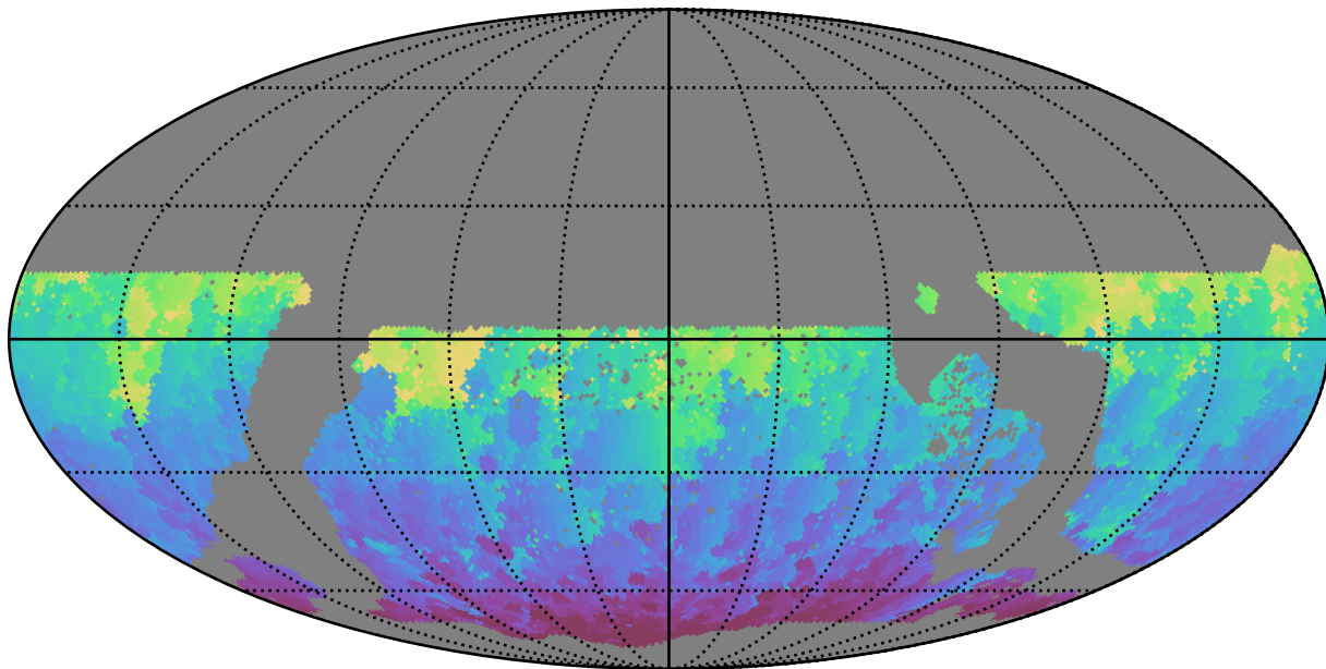
too_elab_r8_d2_giz_v3.4_10yrs WFD g band: Min HA
