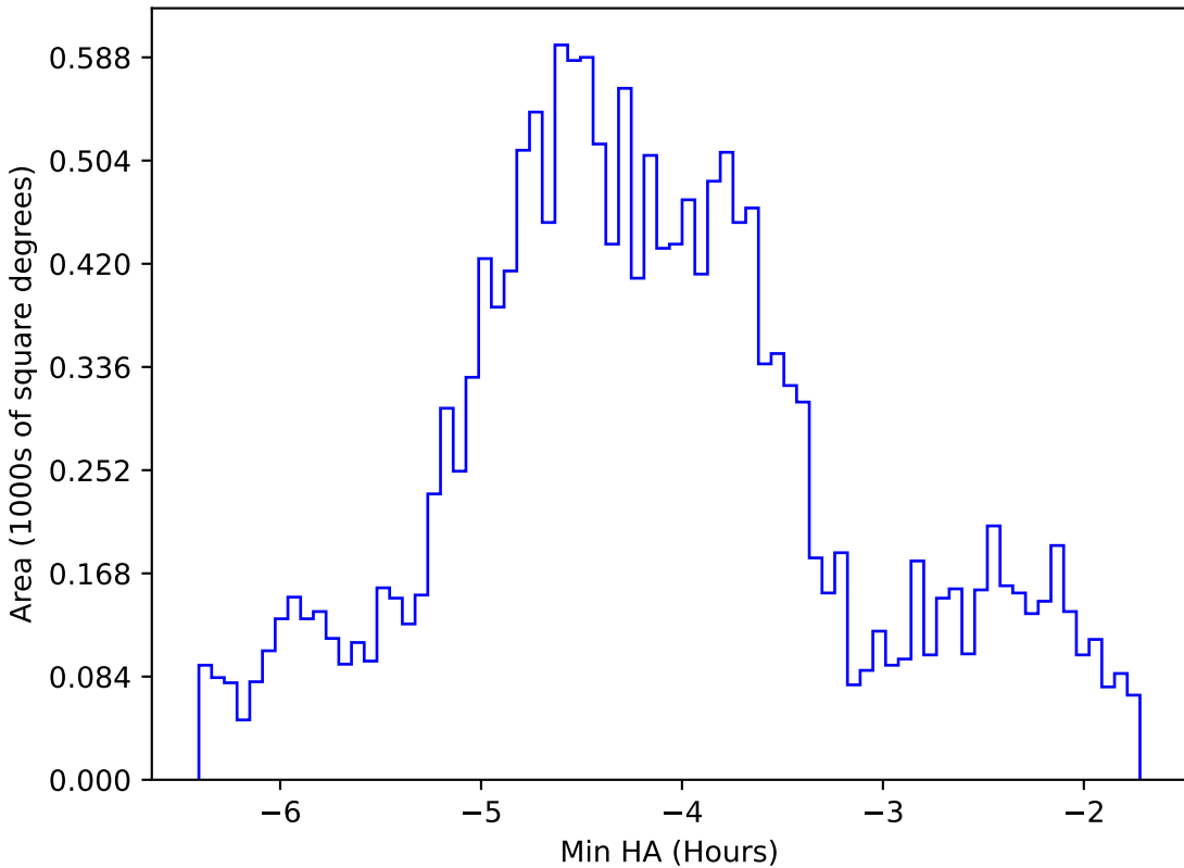
too_elab_r8_d2_giz_v3.4_10yrs WFD g band: Min HA
