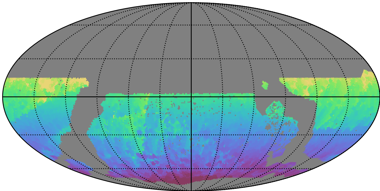
too_elab_r8_d2_giz_v3.4_10yrs WFD all bands: Min HA
