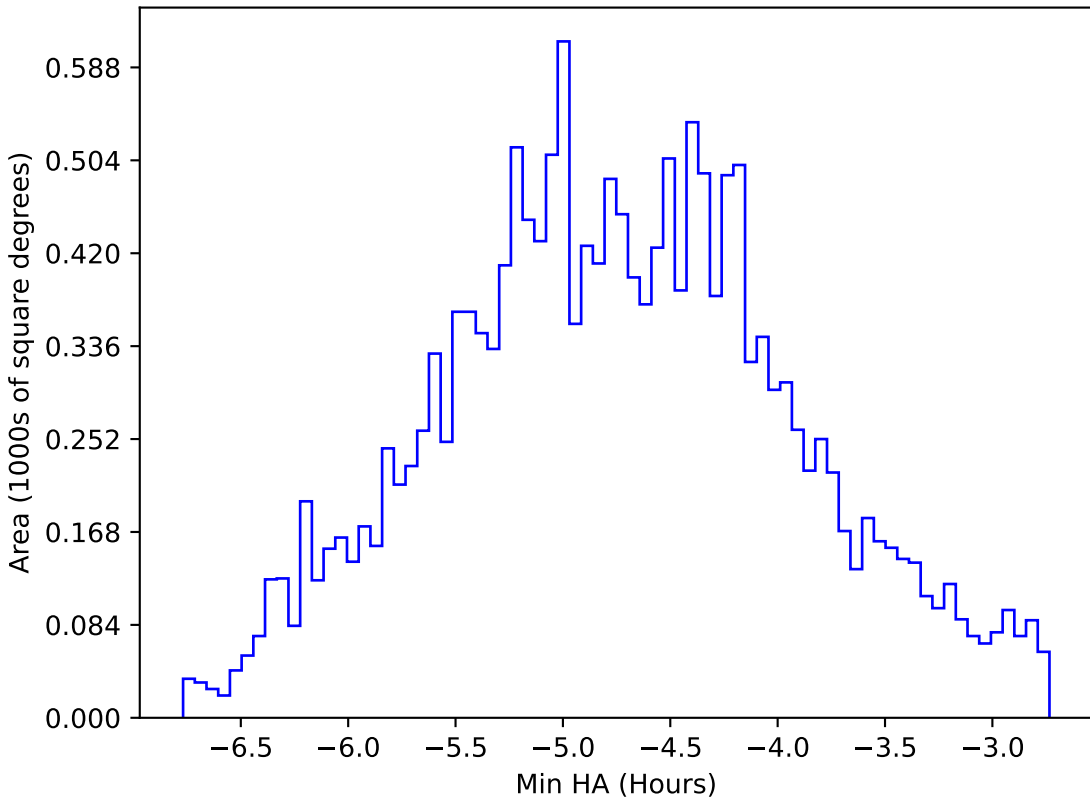
too_elab_r8_d2_giz_v3.4_10yrs WFD all bands: Min HA
