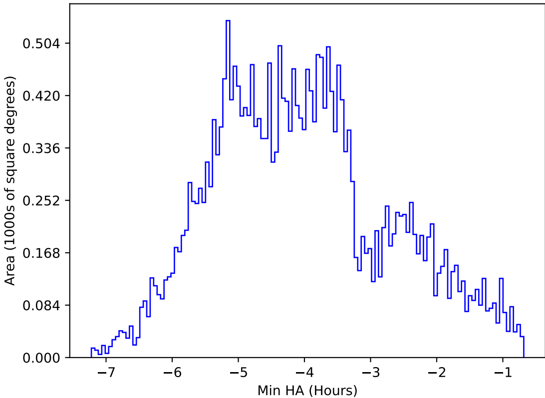
too_elab_r8_d2_giz_v3.4_10yrs All sky z band: Min HA
