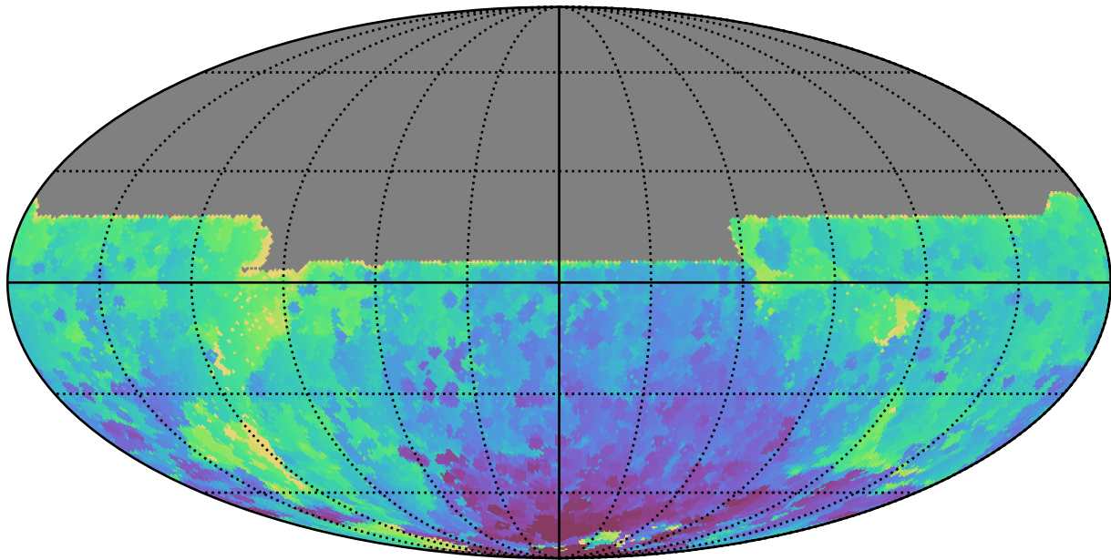
too_elab_r8_d2_giz_v3.4_10yrs All sky y band: Min HA
