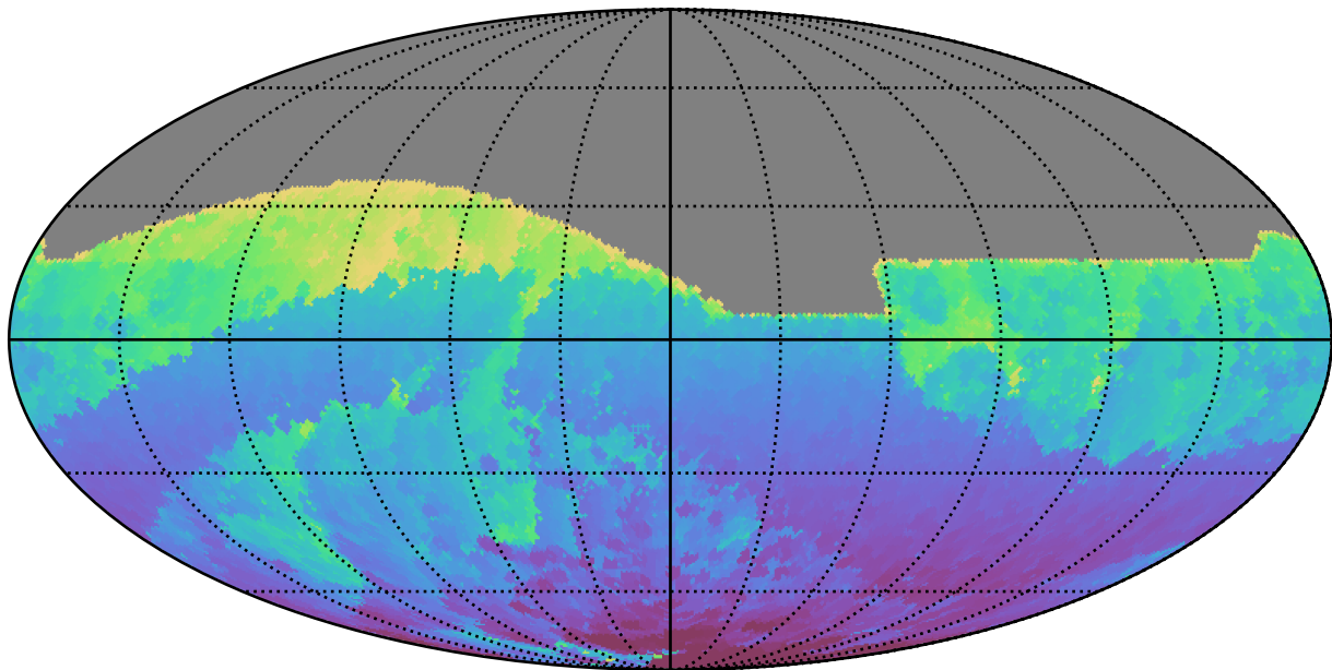
too_elab_r8_d2_giz_v3.4_10yrs All sky r band: Min HA
