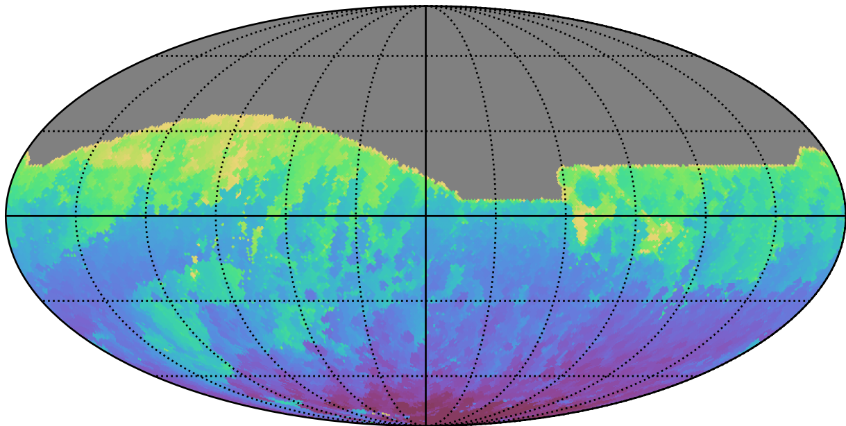
too_elab_r8_d2_giz_v3.4_10yrs All sky i band: Min HA
