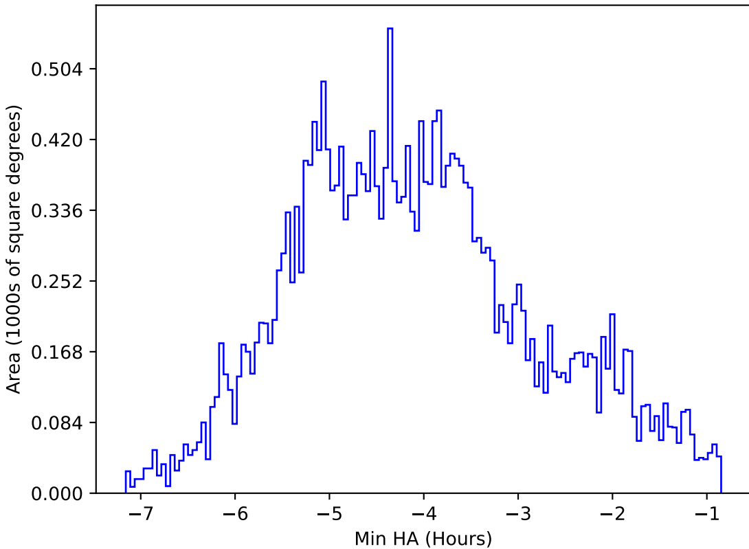
too_elab_r8_d2_giz_v3.4_10yrs All sky i band: Min HA
