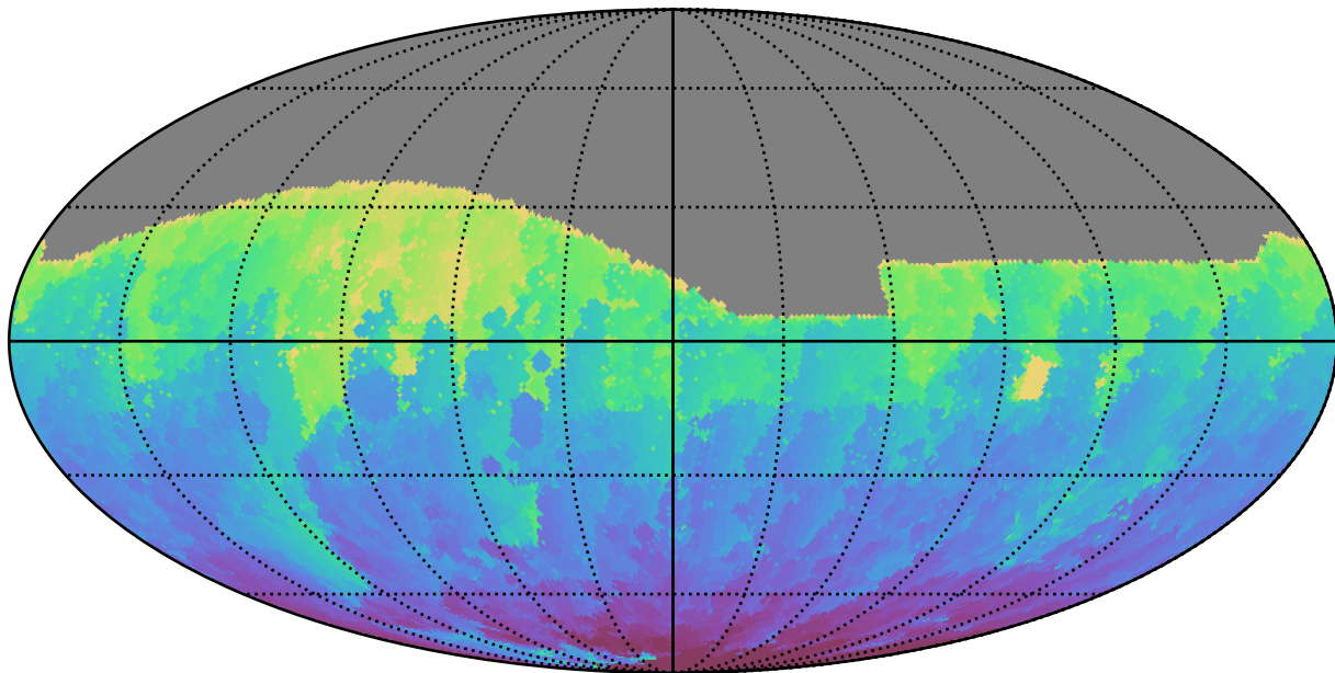
too_elab_r8_d2_giz_v3.4_10yrs All sky g band: Min HA
