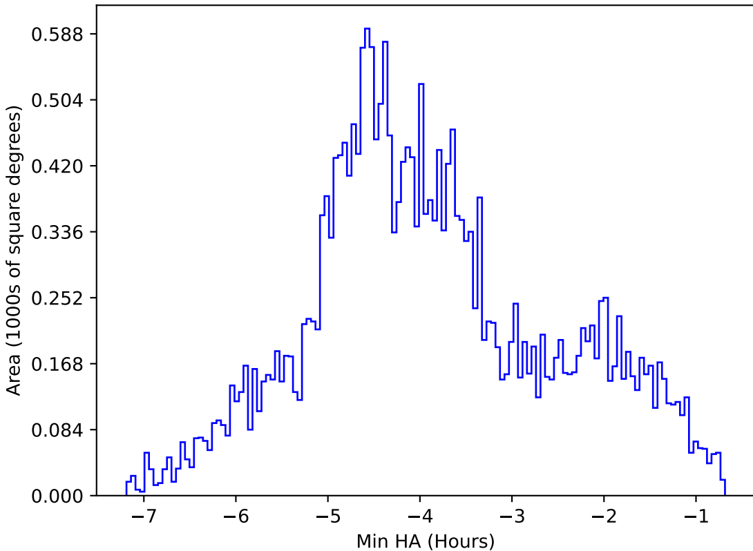
too_elab_r8_d2_giz_v3.4_10yrs All sky g band: Min HA
