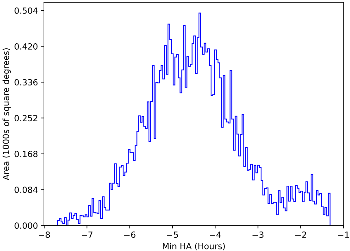
too_elab_r8_d2_giz_v3.4_10yrs All sky all bands: Min HA
