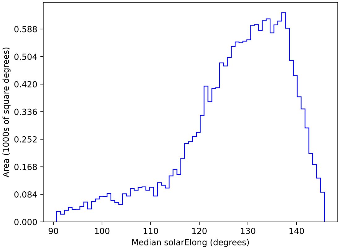
too_elab_r8_d2_giz_v3.4_10yrs WFD z band: Median solarElong
