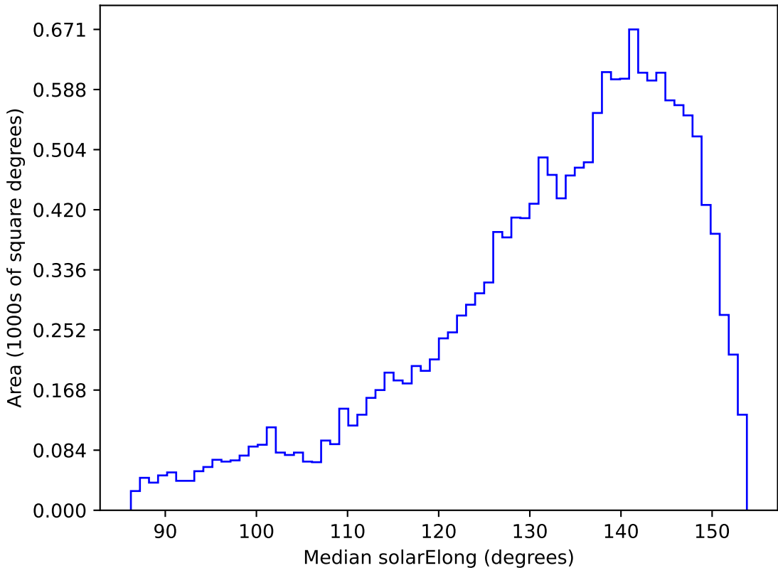
too_elab_r8_d2_giz_v3.4_10yrs WFD u band: Median solarElong
