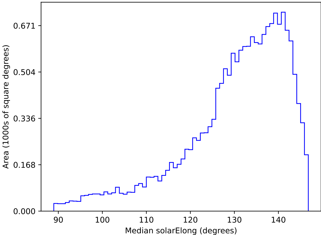
too_elab_r8_d2_giz_v3.4_10yrs WFD r band: Median solarElong
