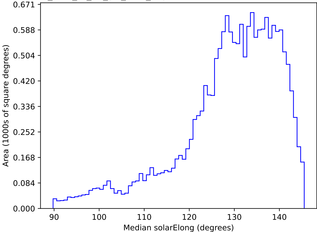
too_elab_r8_d2_giz_v3.4_10yrs WFD i band: Median solarElong
