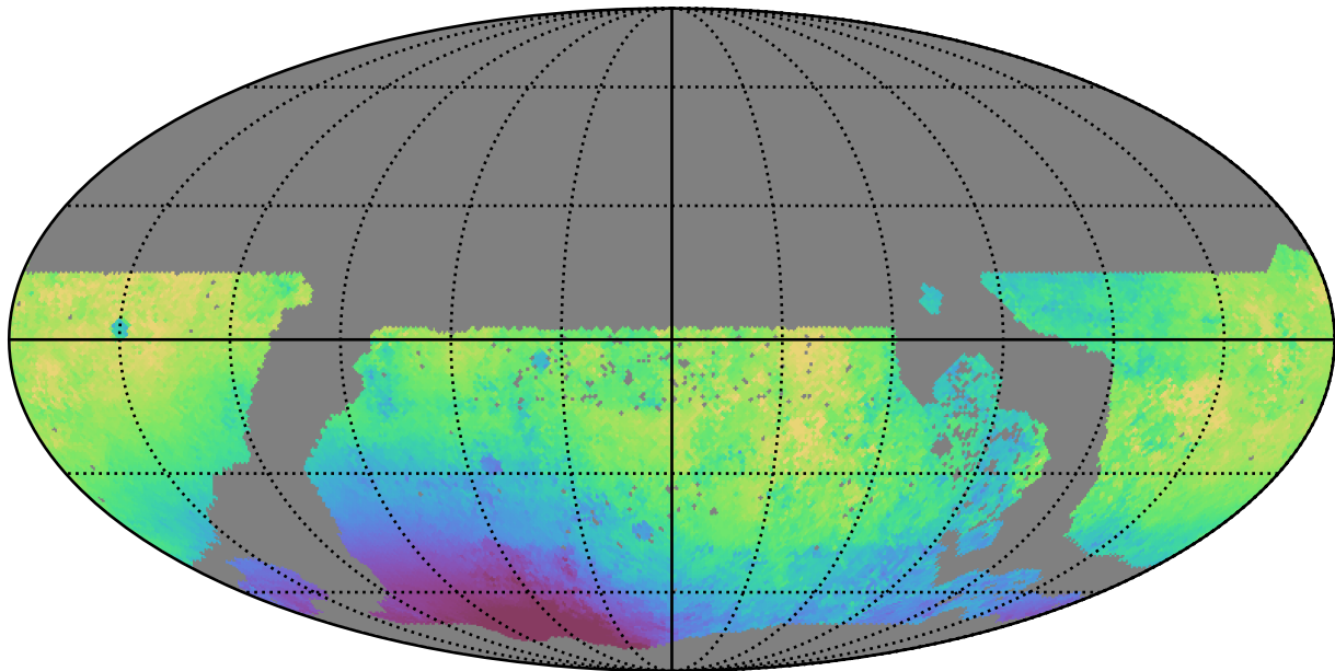
too_elab_r8_d2_giz_v3.4_10yrs WFD g band: Median solarElong
