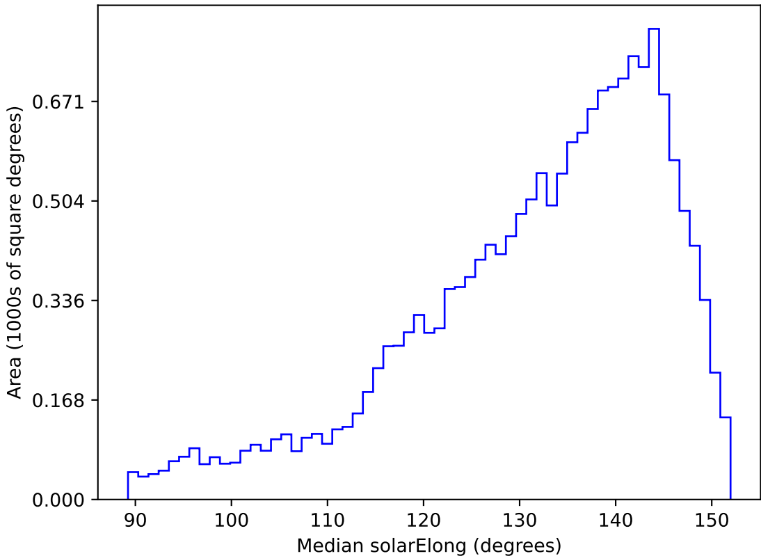
too_elab_r8_d2_giz_v3.4_10yrs WFD g band: Median solarElong
