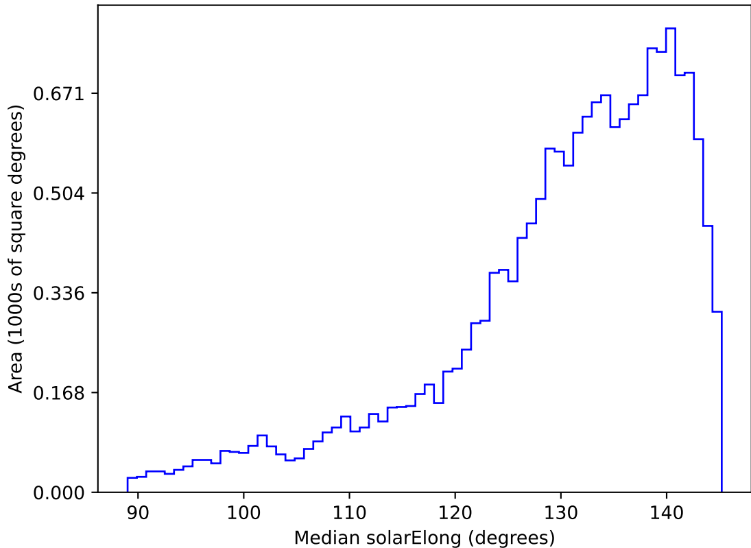
too_elab_r8_d2_giz_v3.4_10yrs WFD all bands: Median solarElong
