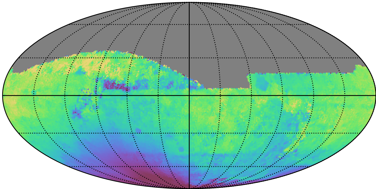
too_elab_r8_d2_giz_v3.4_10yrs All sky z band: Median solarElong
