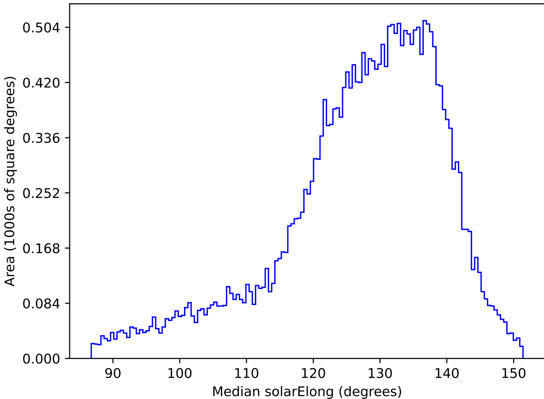
too_elab_r8_d2_giz_v3.4_10yrs All sky z band: Median solarElong
