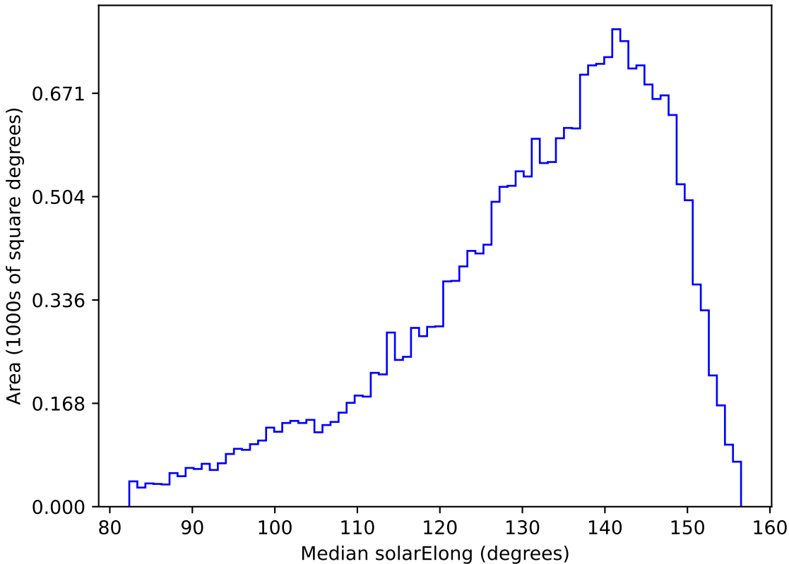
too_elab_r8_d2_giz_v3.4_10yrs All sky u band: Median solarElong
