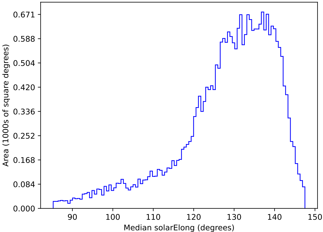
too_elab_r8_d2_giz_v3.4_10yrs All sky i band: Median solarElong
