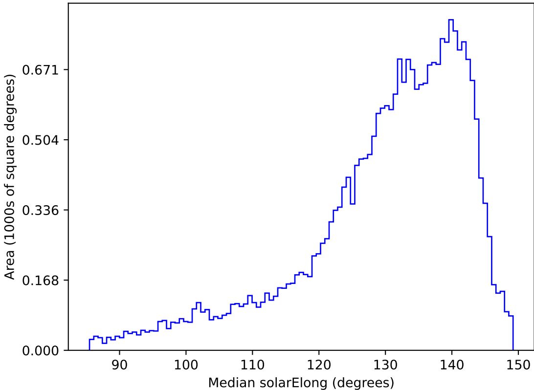
too_elab_r8_d2_giz_v3.4_10yrs All sky all bands: Median solarElong
