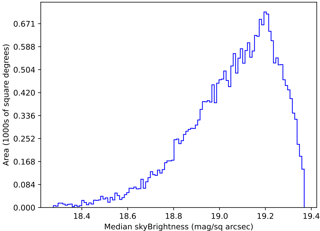
too_elab_r8_d2_giz_v3.4_10yrs Yr 1 z band: Median skyBrightness
