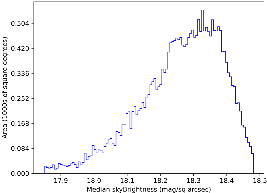
too_elab_r8_d2_giz_v3.4_10yrs Yr 1 y band: Median skyBrightness
