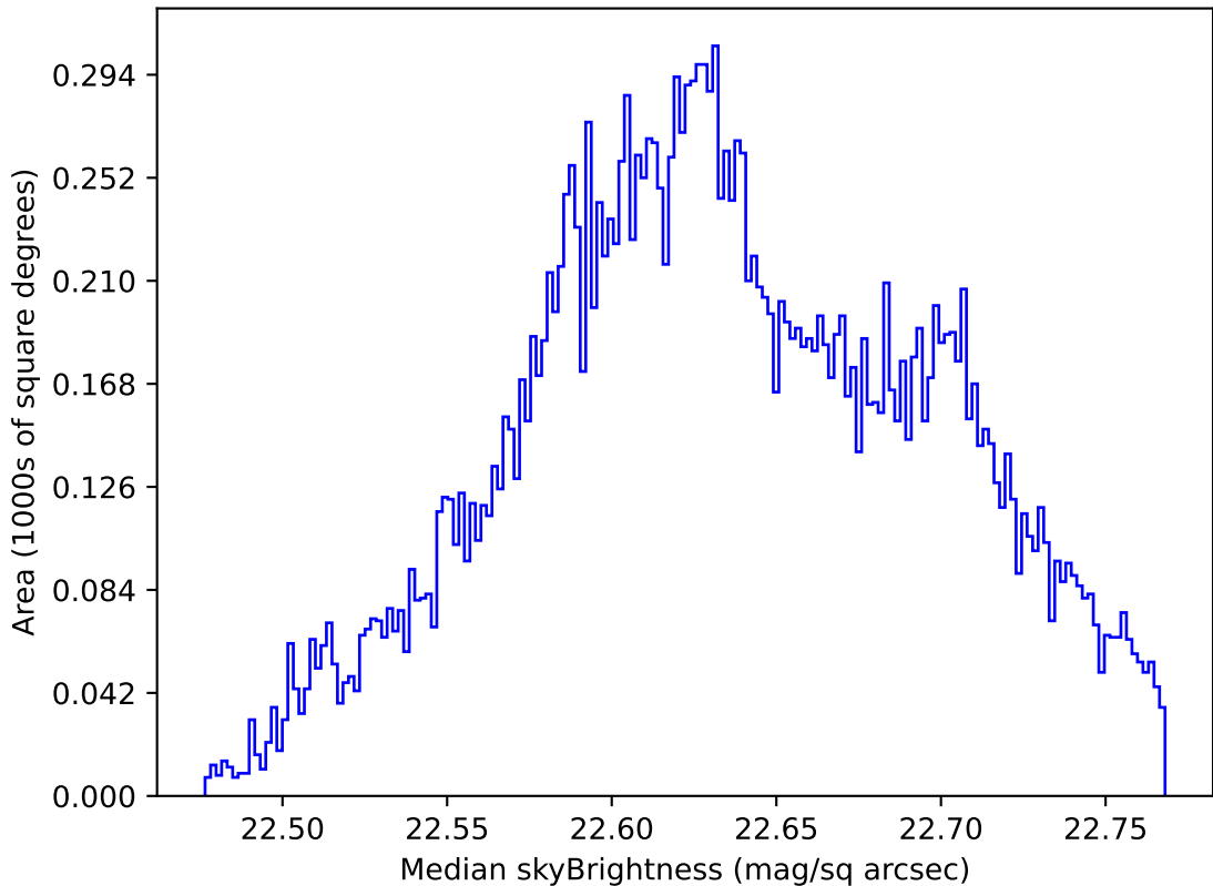
too_elab_r8_d2_giz_v3.4_10yrs Yr 1 u band: Median skyBrightness
