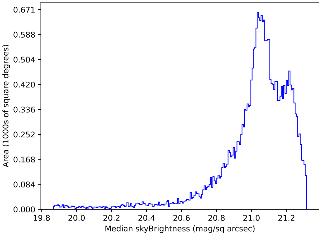
too_elab_r8_d2_giz_v3.4_10yrs Yr 1 r band: Median skyBrightness
