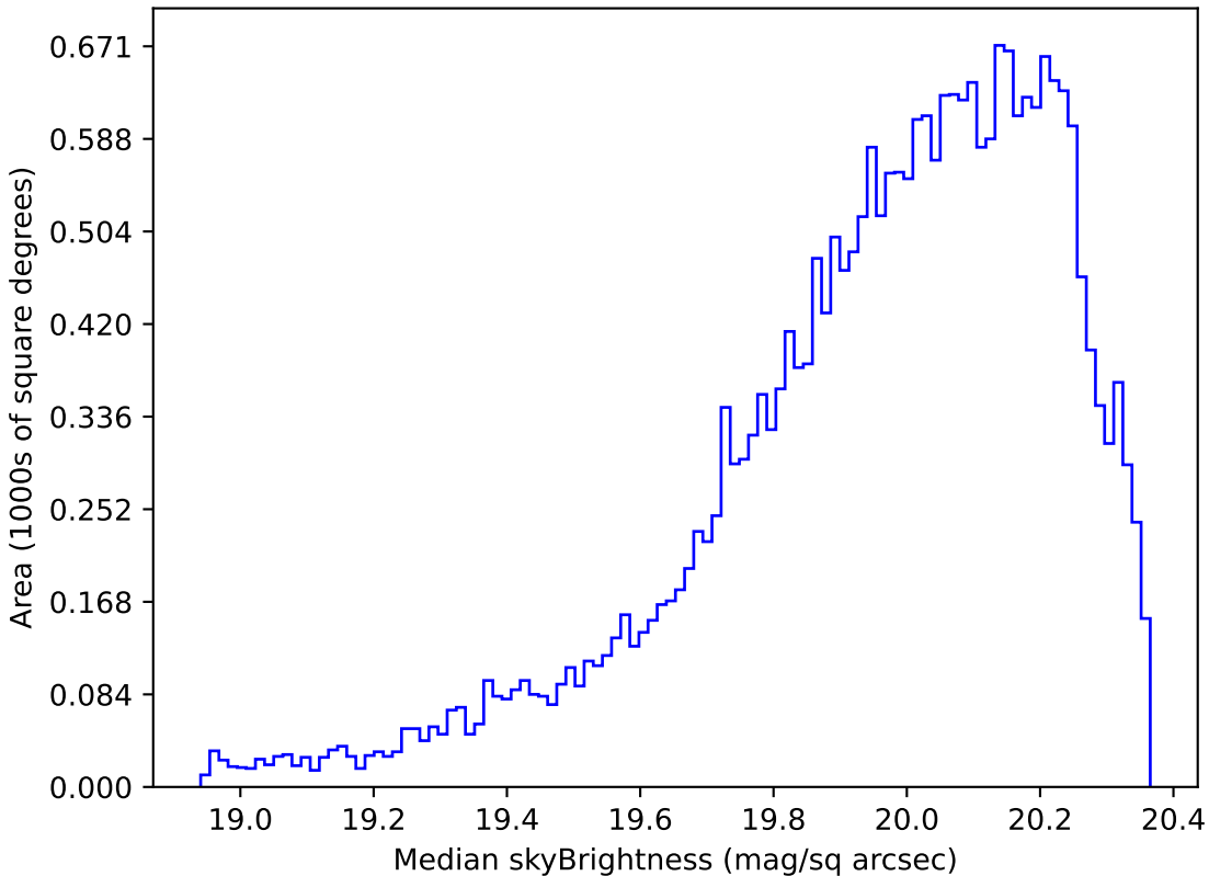
too_elab_r8_d2_giz_v3.4_10yrs Yr 1 i band: Median skyBrightness
