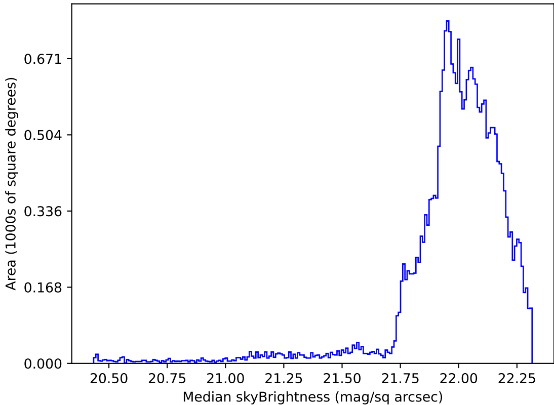
too_elab_r8_d2_giz_v3.4_10yrs Yr 1 g band: Median skyBrightness
